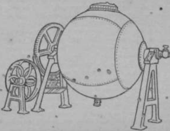
Flo. 1"—SPHERICAL RAG-BOILER.
