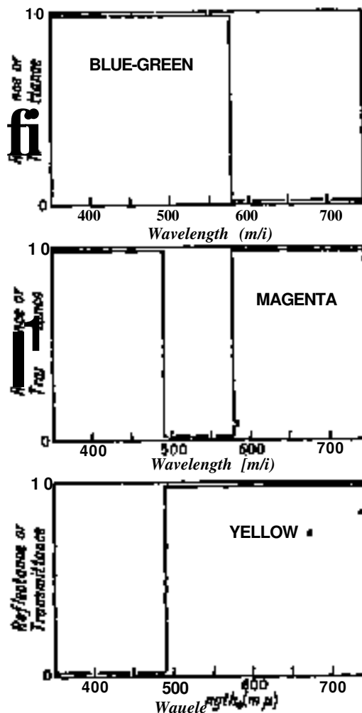
FIG. 9.—IDEAL REFLECTANCE OR TRANSMITTANCE CURVES OF SUBTRACTIVE COLOURANTS IN FULL CONCENTRATION.
