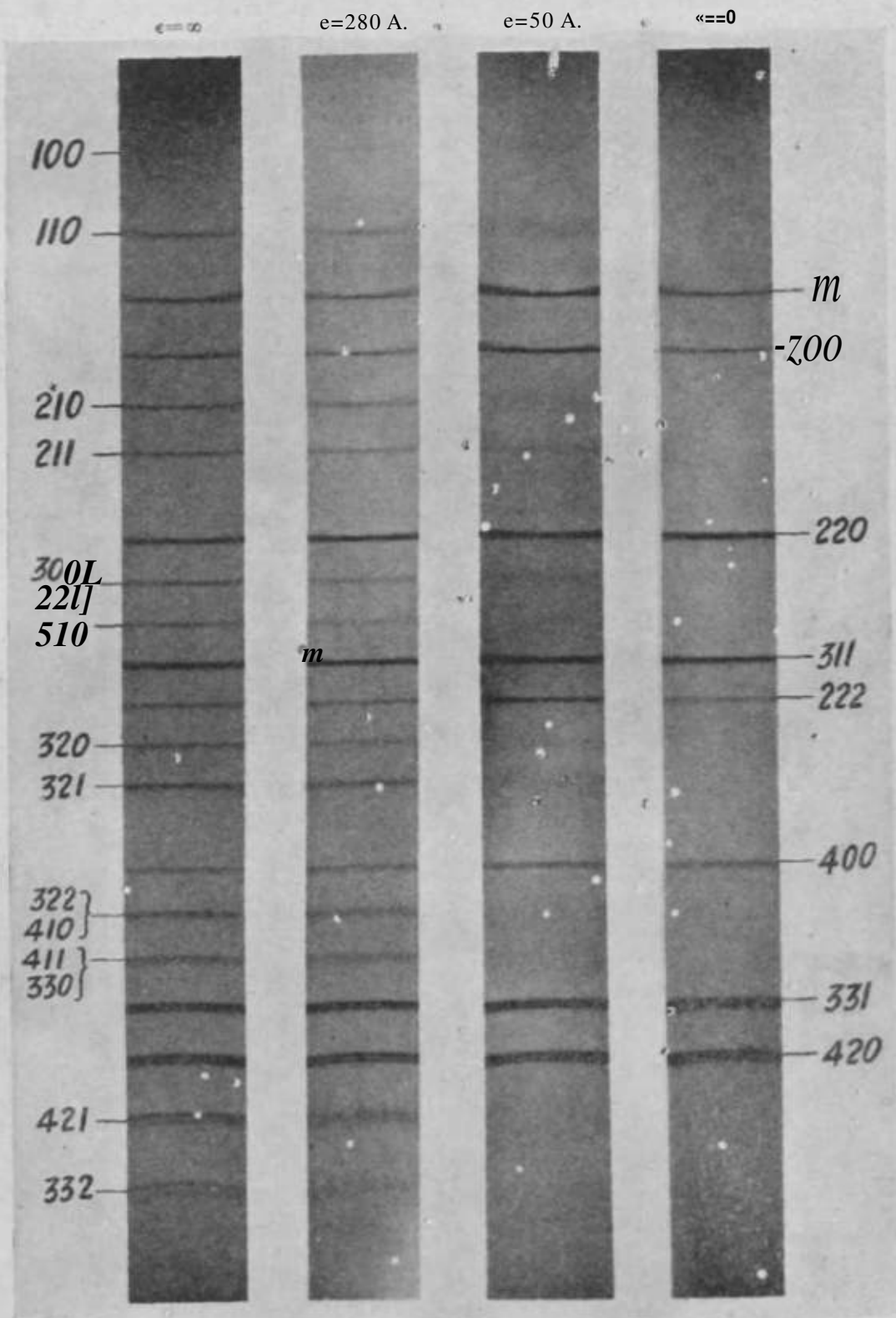
FLO. 10.—POWDER PHOTOBAPHS of \text{Cu}_a\text{Au} . «=Siz6 of anti-phase nviolei. (From Jones and Sykes, Proc. Roy. Soc. 1 , 1938, A, 166, Plate 1ft.)
