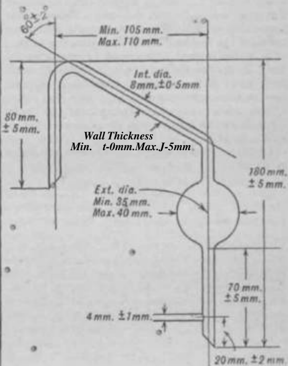
FIG. 3.—STILL HEAD FOR POLBNSKE DISTILLATION APPARATUS.
