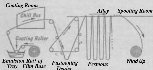
FIG. 2.—DIAGRAM OF FILM EMULSION COATING PLANT.
