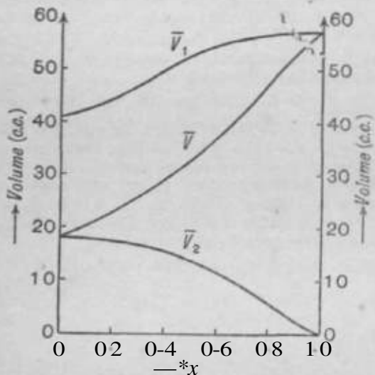
FIG. 2.—THE PARTIAL MOLAR VOLUME OF PERCHLORIC ACID (ADD THE PARTIAL MOLAR VOLUME OF WATER; V_2 ) AT 15°C.
