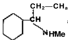
Methyl-α-phenylbutylamine, 0-5.
