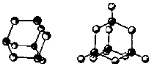
Phosphorus Trioxide.
