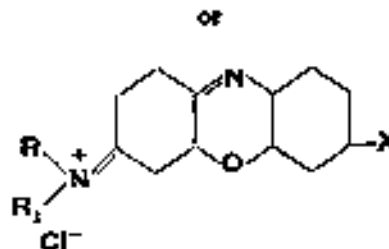
Phenoxazonium or p-quinonoid
