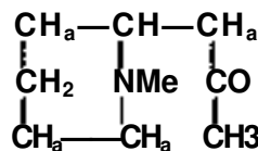
iso -Methylpiperidylpropane.
