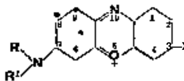
Phenoxazonium or o-quinonoid.
