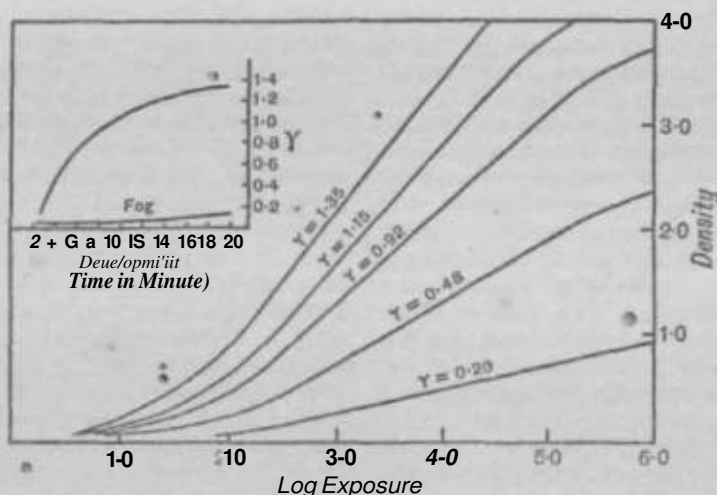
FIG. 5.—FAMHA' OF CHARACTERISTIC CURVES WITH CORRESPONDING \gamma - t AND Fog- t CURVES.
