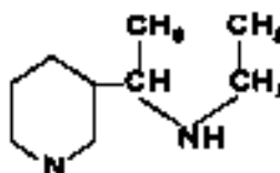
Ethyl-a-(3-pyridyl)ethylamine, 003.
