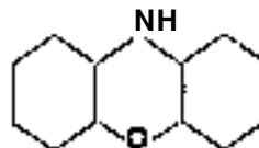
Phenoxazine.
