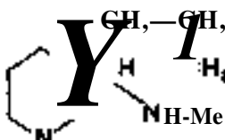
Methyl-a-(0-pyridyl)butylamine, <0-5.
